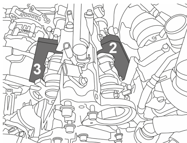
Camshaft setting tool (3+2)
