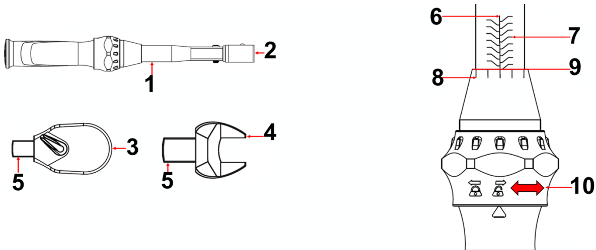
Lowest value 6 Nm
